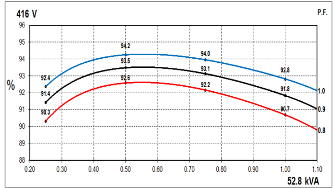
60Hz Curves
