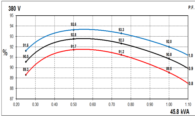
50Hz Curves
